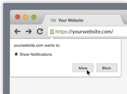
Desktop Opt-in
